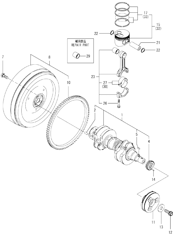
Fig.8. CRANKSHAFT & PISTON
