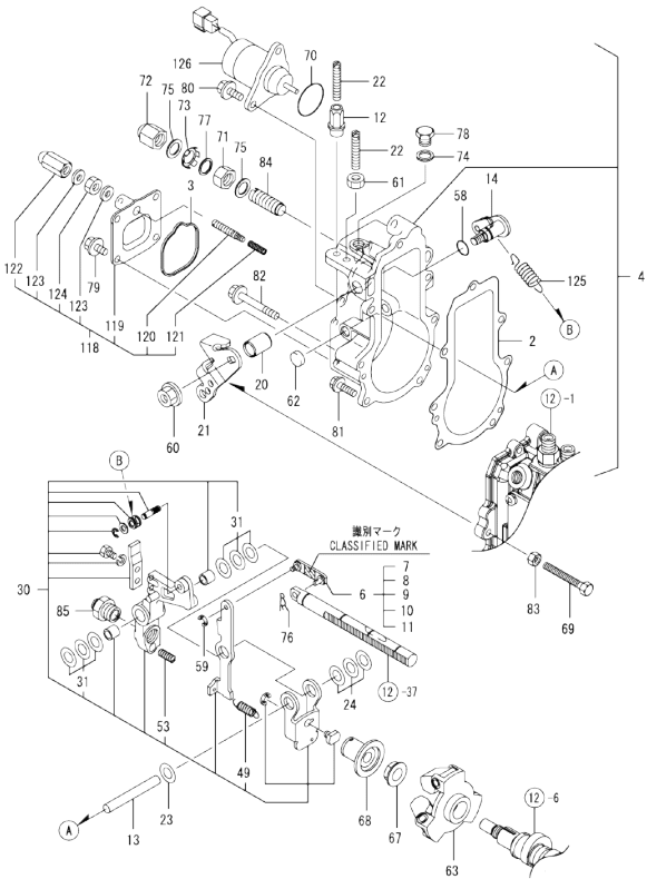
Fig.13. GOVERNOR
