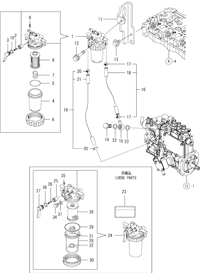
Fig.15. FUEL LINE
